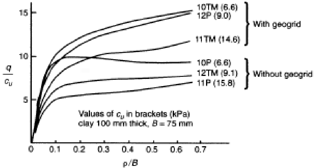
Figure 4.11 Load versus deflection curves for soils with and without geogrid reinforcement
